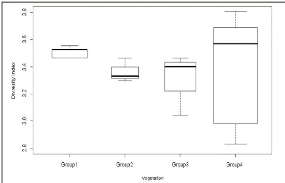
Figure 5: Boxplot showing the diversity index in the four communities identified by Agglomerative Hierarchical Clustering (AHC).
