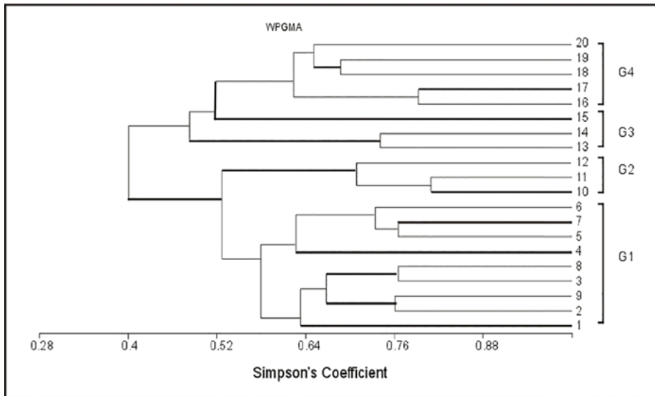
Figure 3: Dendrogram obtained from Agglomerative Hierarchical Clustering (AHC) for 20 sites (Qualitative data).
