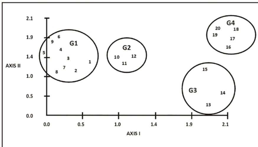
Figure 4: DECORANA (axes 1 & 2) plot of the 20 sites from study area. Circles are plotted as overlay of four associations, segregated by the Agglomerative Hierarchical Clustering (AHC).
