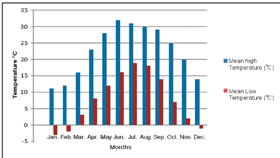
Figure 2: Average high and average low annual temperature in (°C) of the study area (data from nearby metrological station, Abbottabad).
